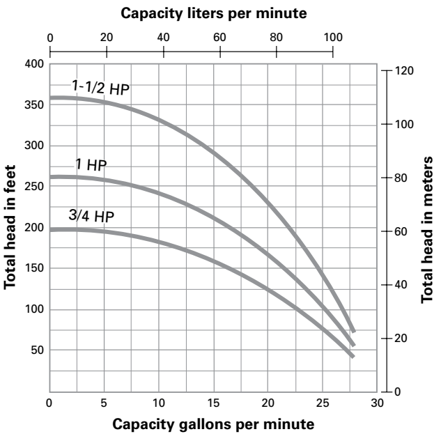
PUMP PERFORMANCE – 20 GPM
